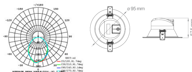
LUMINOUS INTENSITY DISTRIBUTION DIAGRAM
